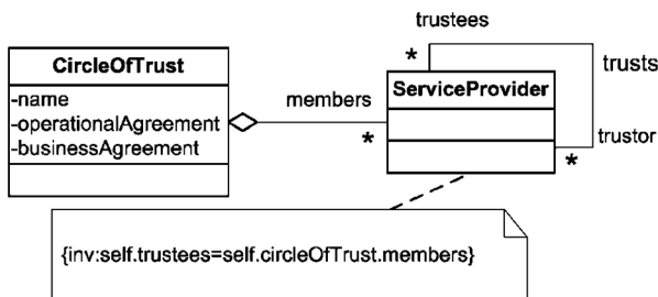
Fig. 4. Circle of Trust pattern (from [39]).
