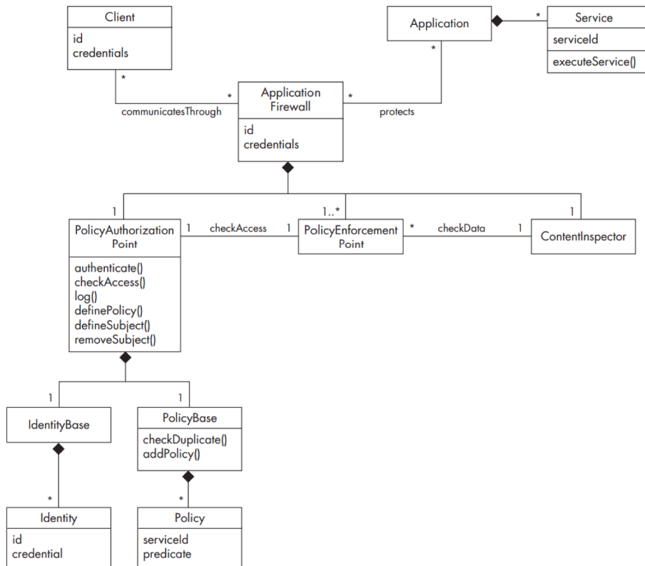
Fig. 2. Class diagram of the Application Firewall pattern (from [7]).
