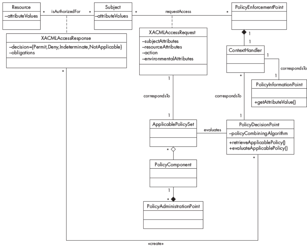
Fig. 3. XACML Access Control Evaluation pattern (from [37]).
