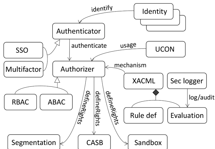
Fig. 5. Patterns used in ZTA.
