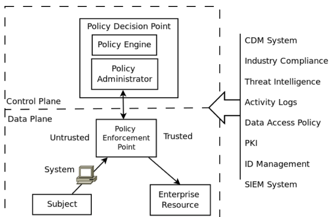
Fig. 1. NIST's conceptual ZTA model.
