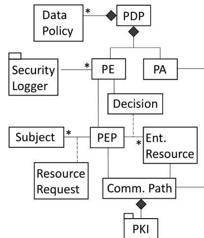
Fig. 6. A preliminary SRA for ZTA.
